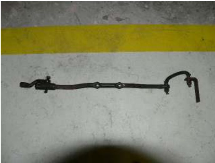
STEERING ARM, CENTER LINK, AND IDLER ARM REMOVED
